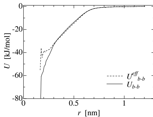
Figure 2. Effective interaction energy between water blobs calculated using AA-MD trajectory in a pure water system. The definitions for U are given in text.
