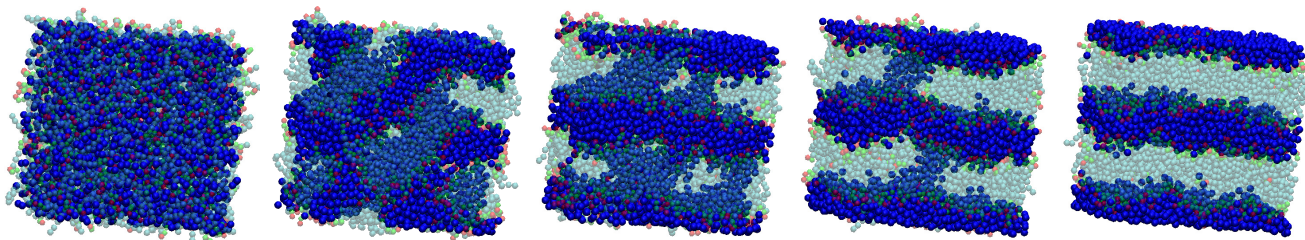
Figure 9. Snapshots of lamellar formation of the C_{12}E_2 /water system from a random initial configuration. The time stamps are 0, 1, 4, 7, and 10 ns from left to right. Water is depicted in blue solid particles, whereas the C_{12}E_2 molecules are drawn in transparent representation. (see Fig. 1) The molecular graphics are created with VMD(29).
