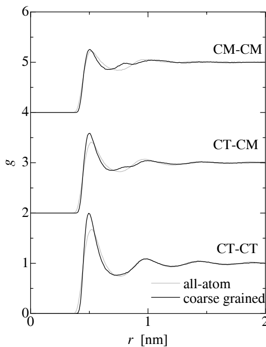
Figure 5. Radial distribution functions in the pure dodecane system.
