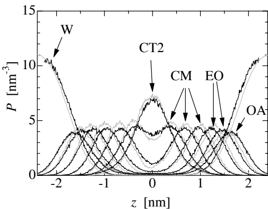
Figure 8. Density profile of the CG segments along the C_{12}E_2 bilayer normal. CG-MD and AA-MD results are given in black and grey lines, respectively.
