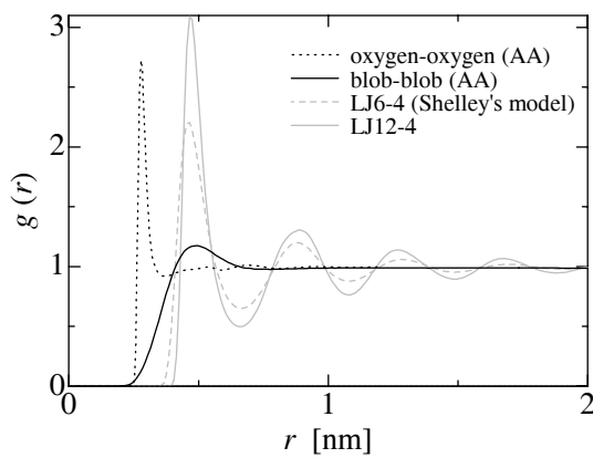
Figure 3. Radial distribution function for pure water systems. Black lines show AA-MD results; grey lines show CG-MD.
