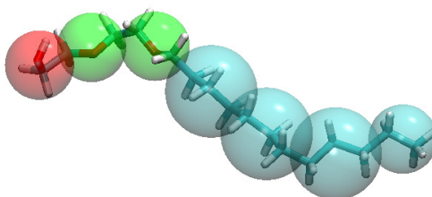
Figure 1. Coarse-grained molecular model for C_{12}E_2 . Transparent spheres represent coarse-grained particles. The molecular graphics are created with VMD(29)
