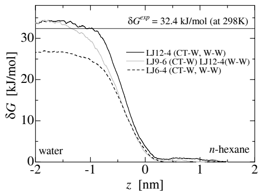
Figure 7. Free energy profile of a hexane molecule across the hexane/water interface.
